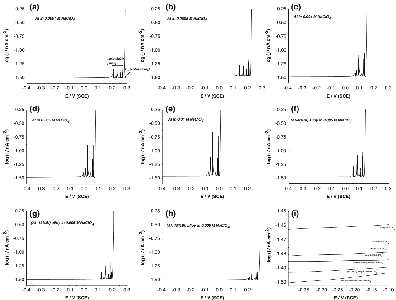
Fig. 1 Potentiodynamic anodic polarization curves recorded for pure Al in NaClO 4 solution of various concentrations ( 10^{-4} – 10^{-2} M) (a–e), for (Al + 6%Si), (Al + 12%Si), and (Al + 18%Si) alloys in 0.005 M NaClO 4 solution (f–h) and for a comparison of the passive
