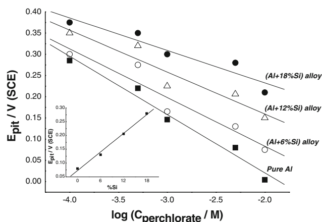
Fig. 2 Dependence of the pitting potential ( E_{\text{pit}} ) on \log C_{\text{perchlorate}} recorded for pure Al, (Al + 6%Si), (Al + 12%Si), and (Al + 18%Si) alloys at 25 °C
