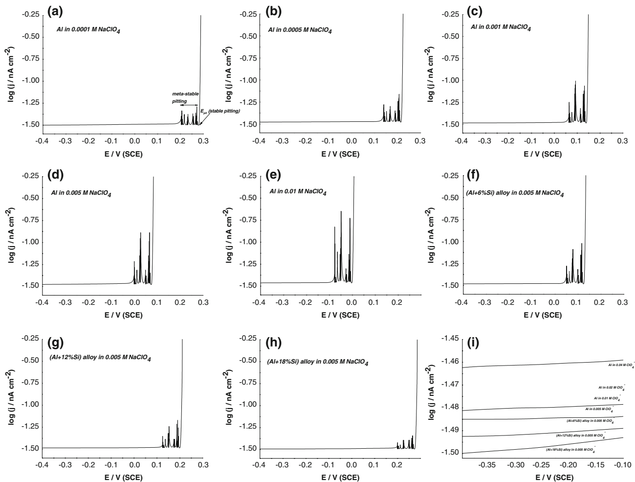
Fig. 1 Potentiodynamic anodic polarization curves recorded for pure Al in NaClO 4 solution of various concentrations (10 -4 –10 -2 M) (a–e), for (Al + 6%Si), (Al + 12%Si), and (Al + 18%Si) alloys in 0.005 M NaClO 4 solution (f–h) and for a comparison of the passive
